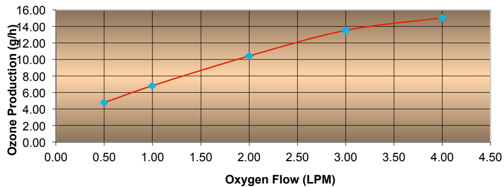
Ozone Production
