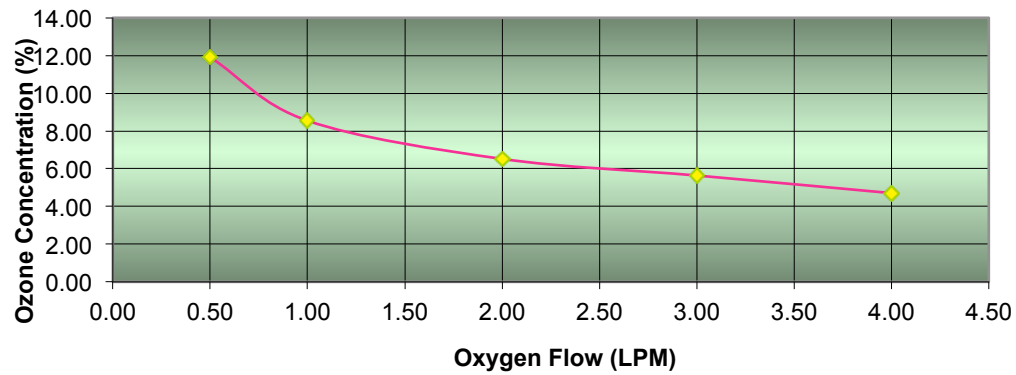
Ozone Concentration
